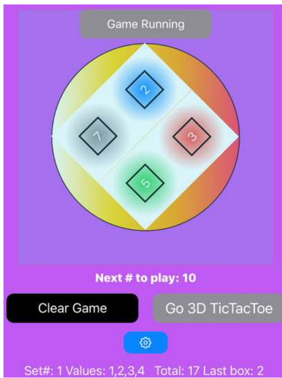
Fig 3. Magic/Antimagic sample
